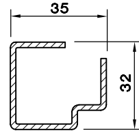
ORTAKAYIT -81/2 DESTEK SAÇI (2.0) 5153.312
