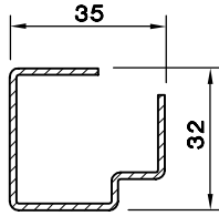
ORTAKAYIT -81/2 DESTEK SAÇI (1.5) 5153.311
