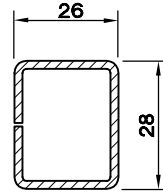
ORTAKAYIT -81/3 DESTEK SAÇI (2.0) 5153.322
