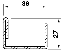
KASA-63/2 DESTEK SAÇI (2.0) 5153.112
