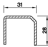
KANAT-56/3 DESTEK SAÇI (2.0) 5153.212
