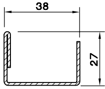
KASA-63/2 DESTEK SAÇI (1.5) 5153.111
